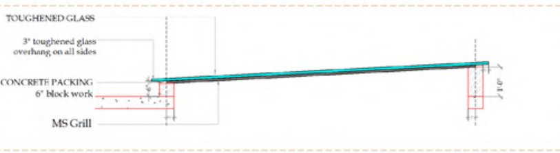
SECTION - A
