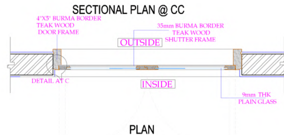
PD - 4'6" X 7'0" - 01 NO'S
