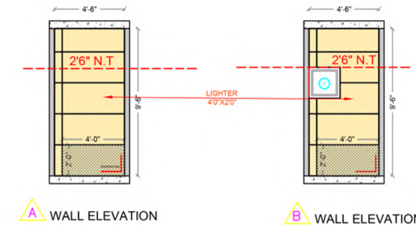
A WALL ELEVATION B WALL ELEVATION
