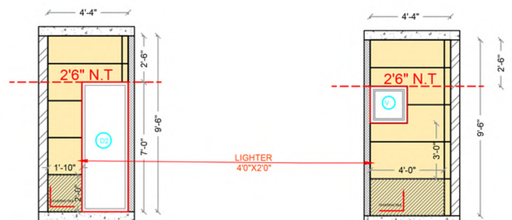
C WALL ELEVATION D WALL ELEVATION
