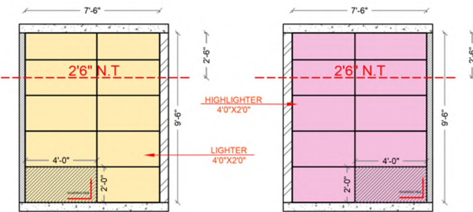
A WALL ELEVATION B WALL ELEVATION
