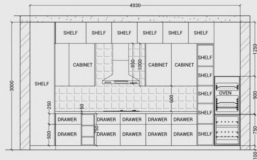
ELEVATION AA'
