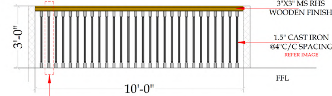
FRONT VIEW
