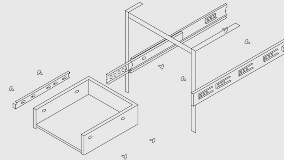
TELESCOPIC DRAWER DETAIL
