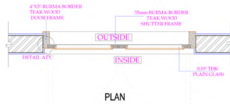
PD - 4'6"X7'0" 01 NO'S
