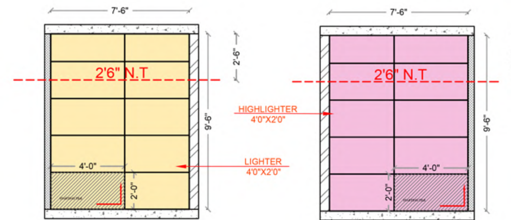
A WALL ELEVATION B WALL ELEVATION
